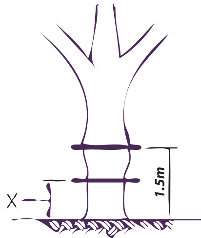
Measurement of stem with irregular swelling made at the narrowest point below the swelling
